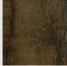
Ash cinder
